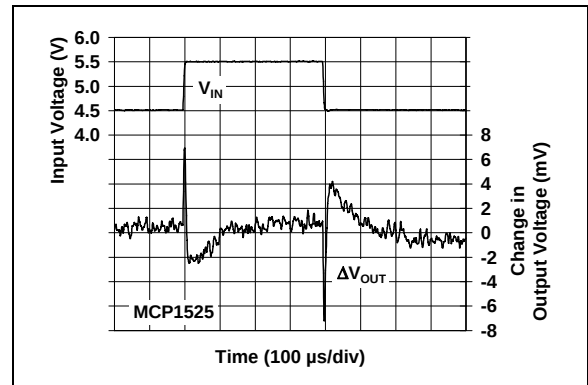
FIGURE 2-17: MCP1525 Line Transient Response.
