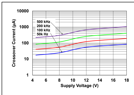
FIGURE 2-6: Crossover Current vs. Supply Voltage.
