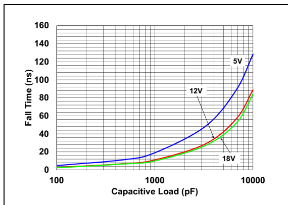
FIGURE 2-4: Fall Time vs. Capacitive Load.
