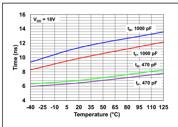
FIGURE 2-5: Rise and Fall Time vs. Temperature.
