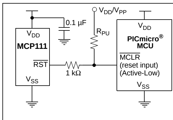
FIGURE 4-4: Typical Application Circuit for PICmicro ® Microcontroller with the ICSP ™ feature.
