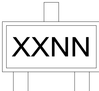
3-Lead SOT-23
