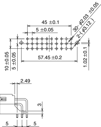
PCB mounting pattern
