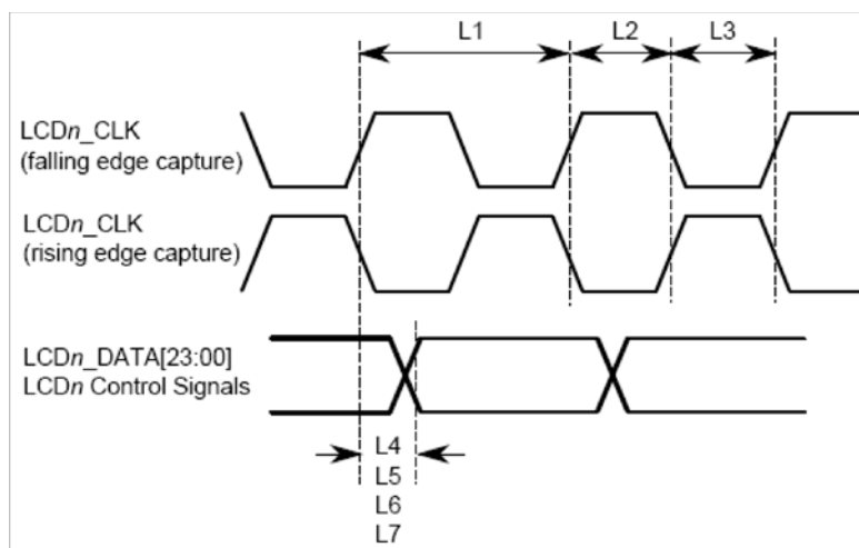
Figure 60. LCD timing
