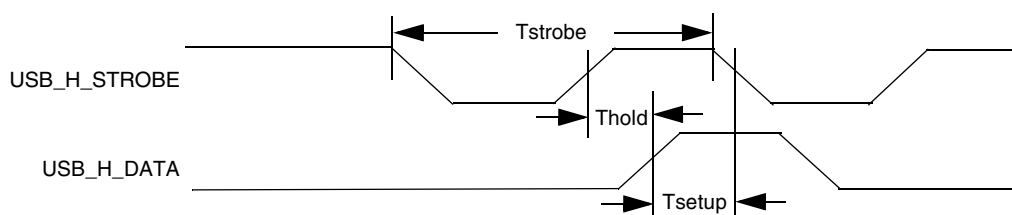
Figure 82. USB HSIC receive waveform
