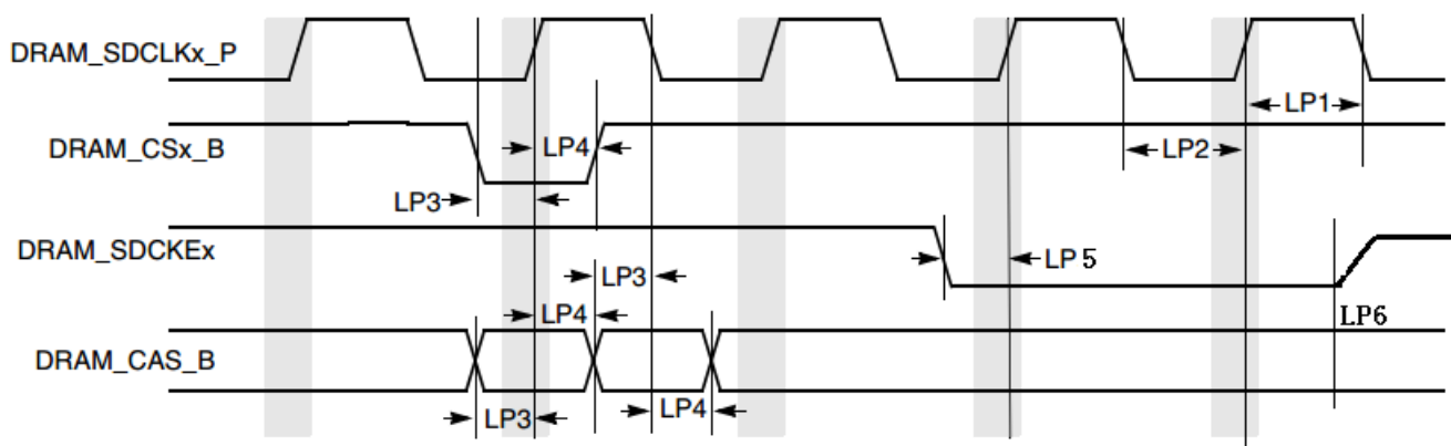
Figure 27. LPDDR3 command and address timing diagram
