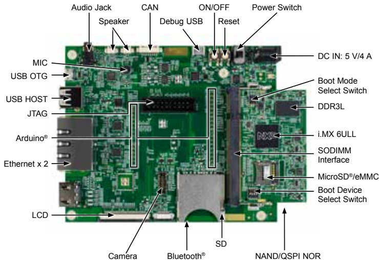
Figure 1: Main interfaces of i.MX 6ULL EVK
