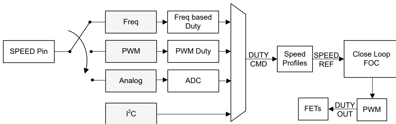
Figure 7-13. Multiplexing the Speed Command
