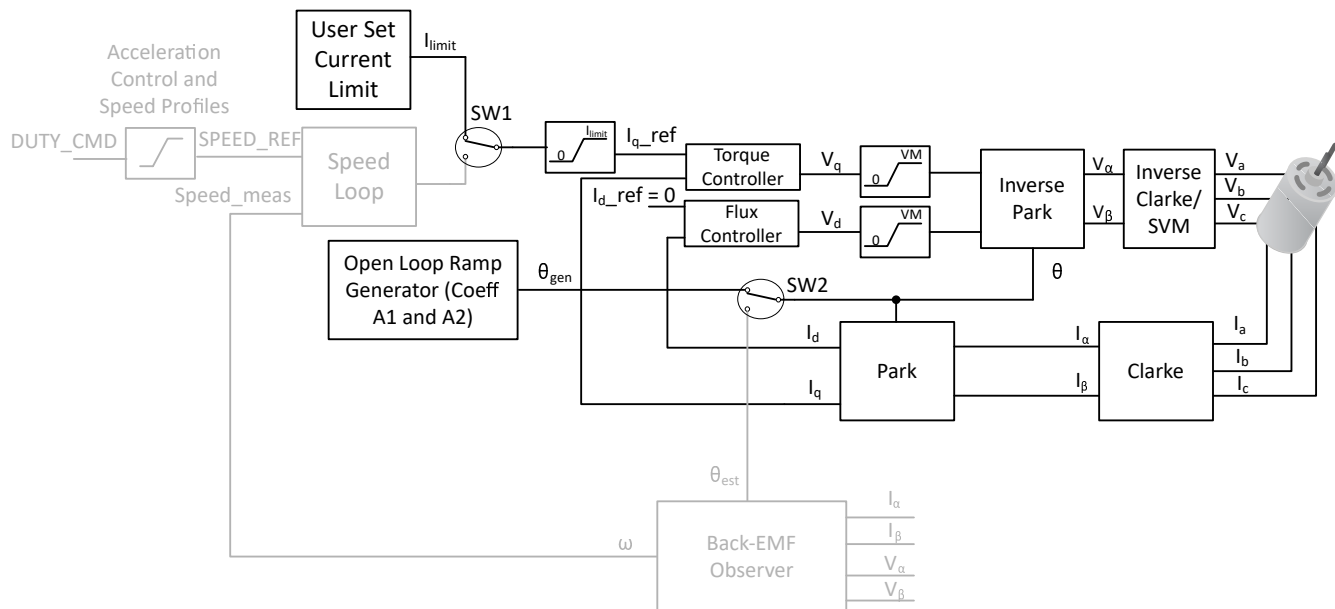
Figure 7-26. Open Loop
