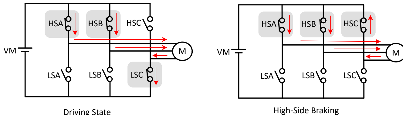
Figure 7-44. High-Side Braking
