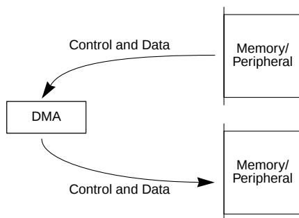
Figure 12-2. Dual-Address Transfer
