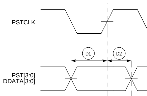
Figure 20-12. Real-Time Trace AC Timing
