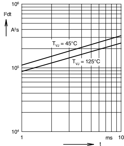
Fig. 5 I^2dt versus time (1-10 ms)
