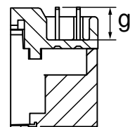
C-C (1:1)
