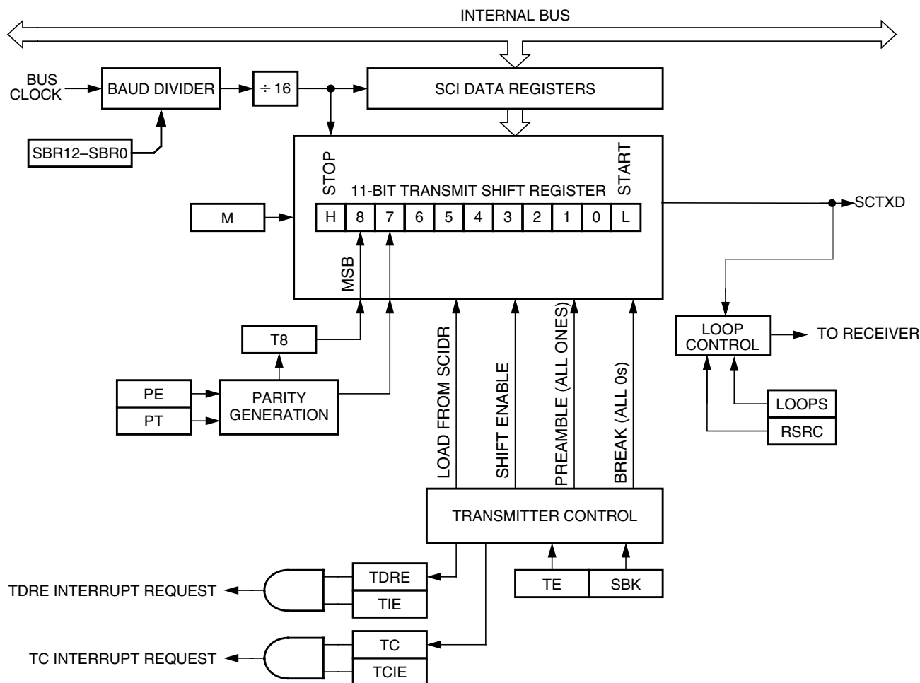
Figure 8-13. Transmitter Block Diagram
