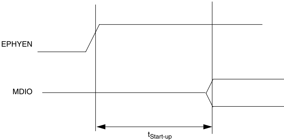
Figure 12-19. EPHY Start-Up Delay
