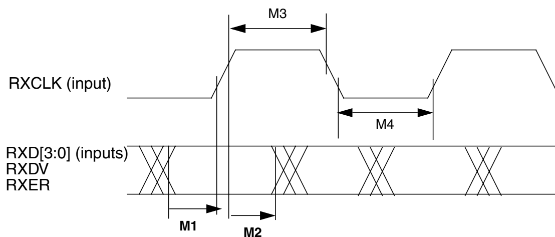
Figure 18-24. MII Receive Signal Timing Diagram
