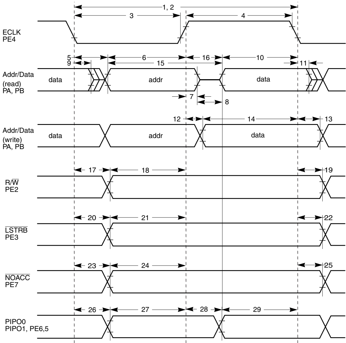
Figure 18-25. General External Bus Timing
