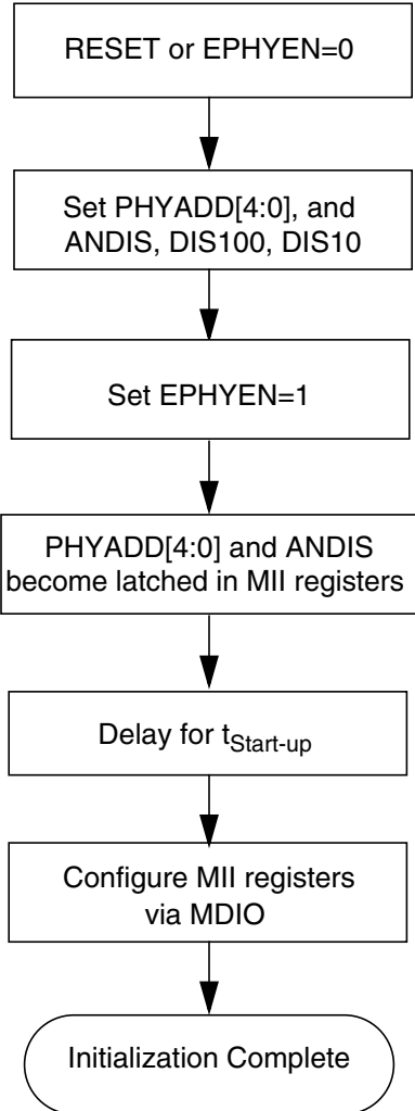
Figure 12-18. EPHY Start-Up / Initialization Sequence
