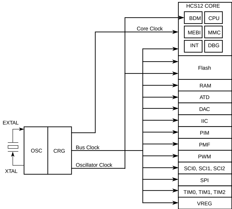
Figure 1-7. Clock Connections
