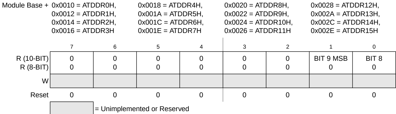
Figure 6-20. Right Justified, ATD Conversion Result Register x, High Byte (ATDDRxH)
