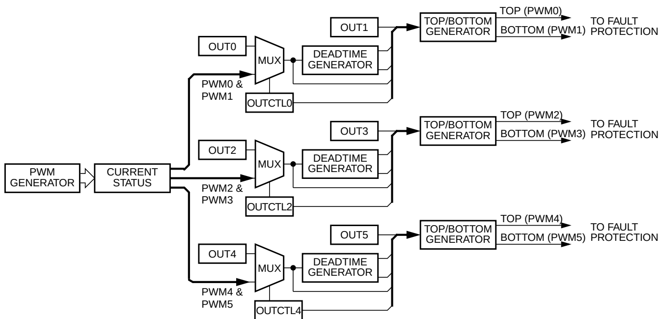
Figure 11-49. Deadtime Generators
