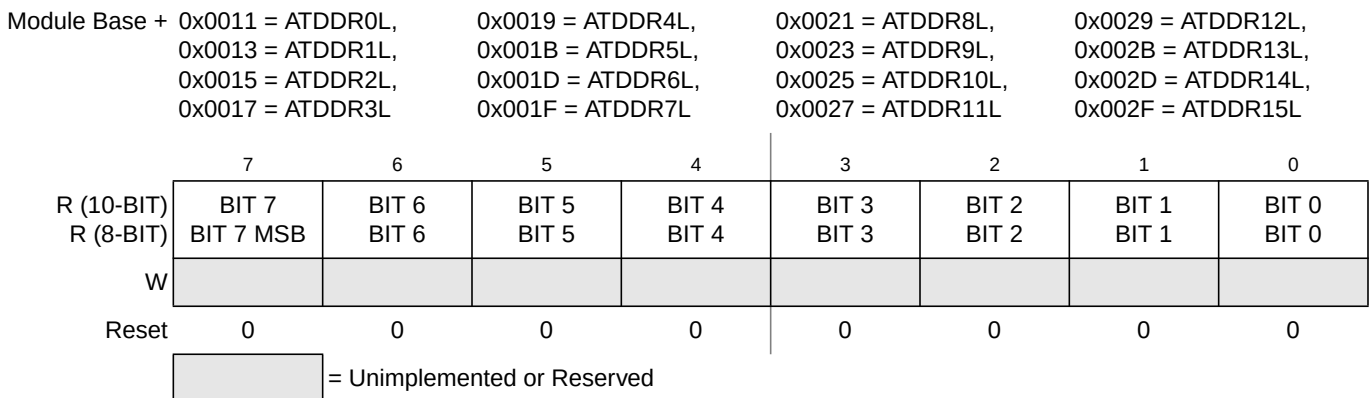
Figure 6-21. Right Justified, ATD Conversion Result Register x, Low Byte (ATDDRxL)
