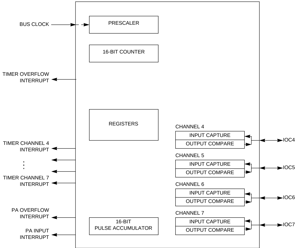
Figure 13-1. Timer Block Diagram
