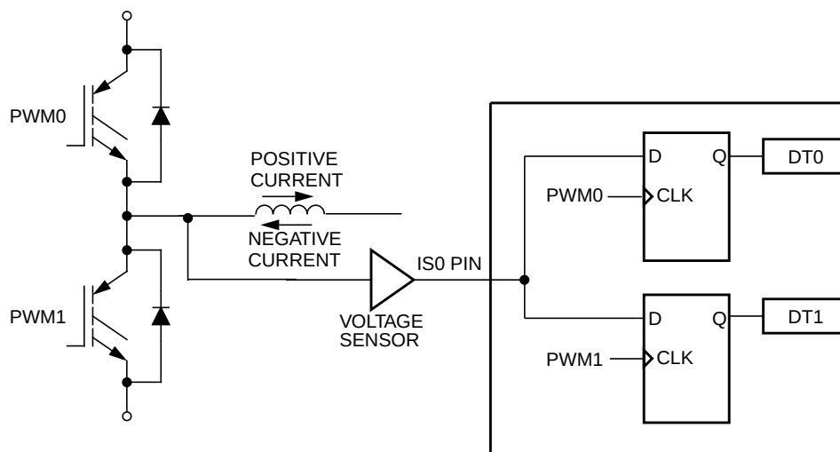
Figure 11-55. Current Status Sense Scheme for Deadtime Correction
