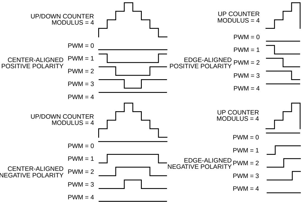
Figure 11-61. PWM Polarity
