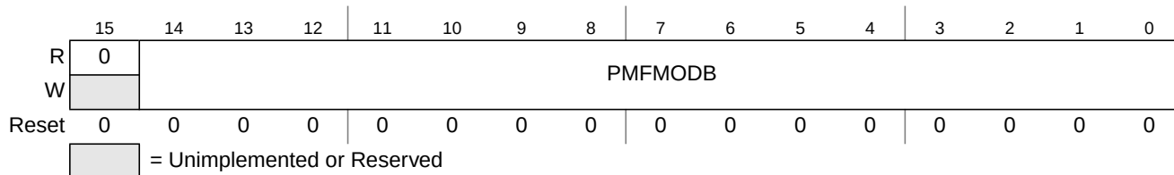
Figure 11-34. PMF Counter Modulo B Register (PMFMOB)
