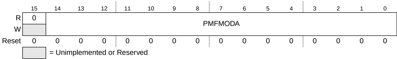
Figure 11-29. PMF Counter Modulo A Register (PMFMODA)
