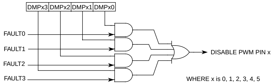
Figure 11-15. Fault Decoder
