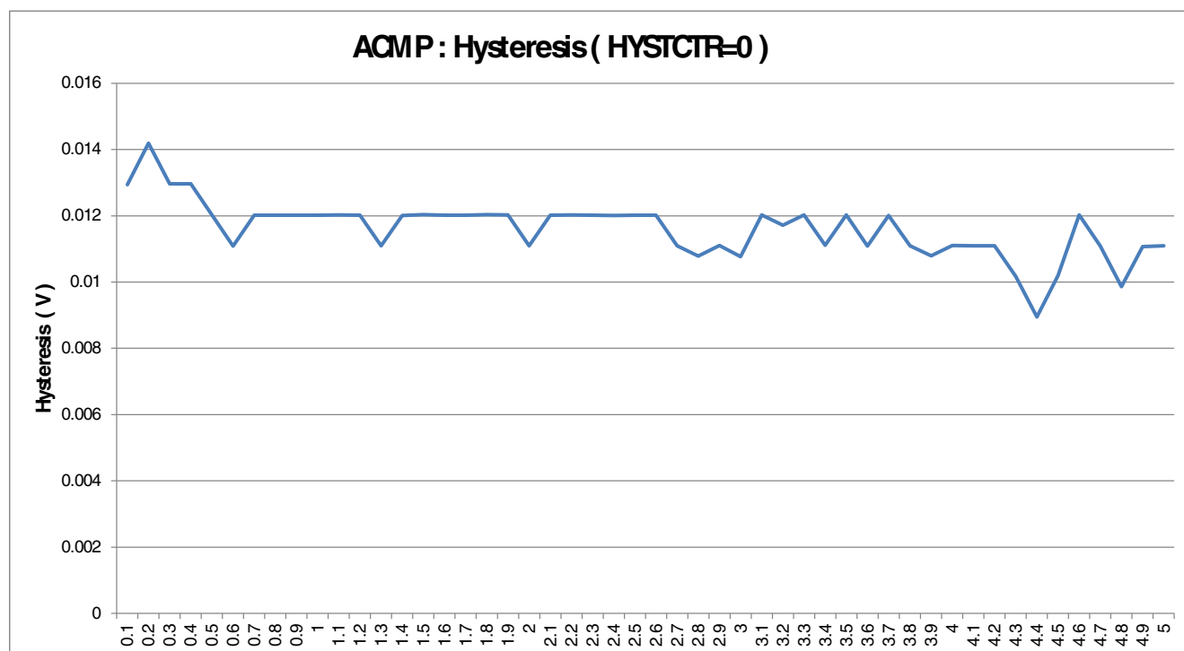
Figure 12. Typical hysteresis vs. Vin level ( V_{\text{DDX}} = 5.0 \text{ V} , PMODE = 0)
