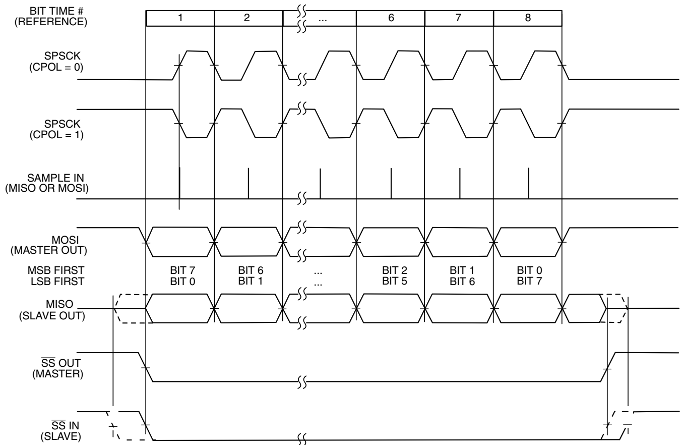
Figure 17-6. SPI clock formats (CPHA = 0)
