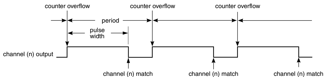
Figure 12-15. EPWM period and pulse width with \text{ELSnB:ELSnA} = 1:0
