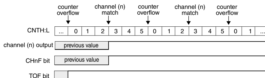
Figure 12-14. Example of the output compare mode when the match sets the channel output
