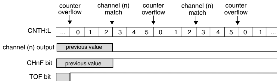
Figure 12-13. Example of the output compare mode when the match clears the channel output
