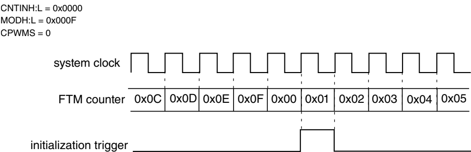
Figure 12-64. Initialization trigger is generated when the FTM counter achieves the value of CNTINH:L
