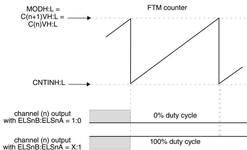
Figure 12-30. Channel (n) output if (C(n)V = C(n+1)V = MOD)
