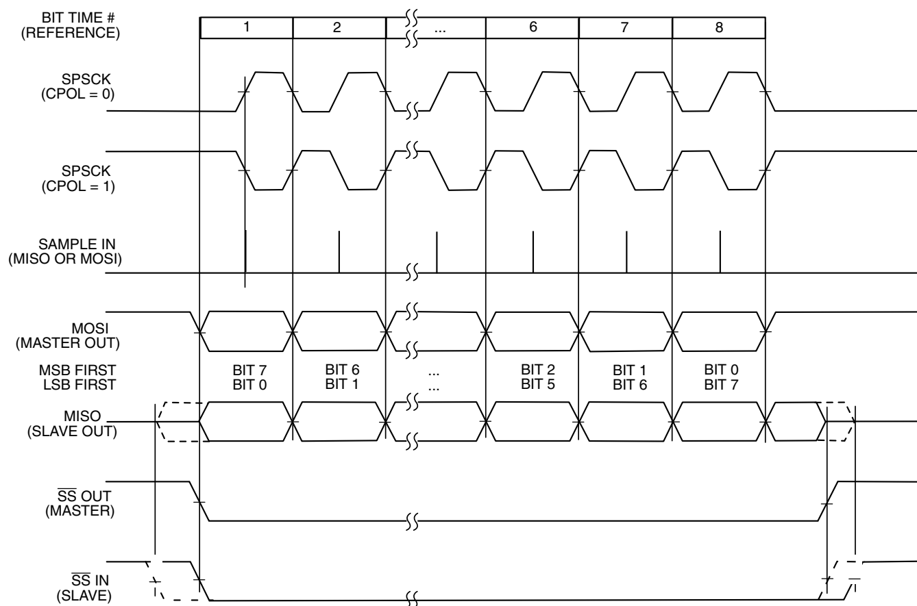
Figure 16-4. SPI Clock Formats ( \text{CPHA} = 0 )
