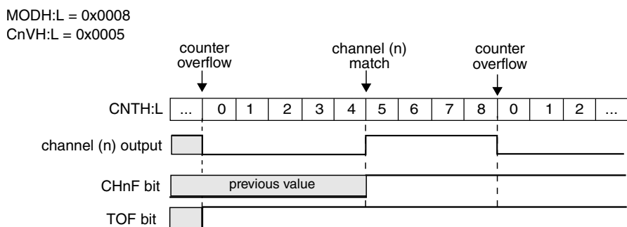
Figure 12-17. EPWM signal with ELSnB:ELSnA = X:1
