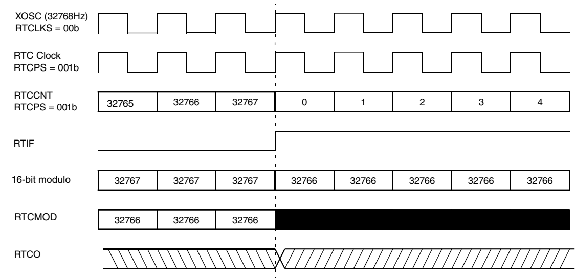
Figure 14-2. RTC counter overflow example
