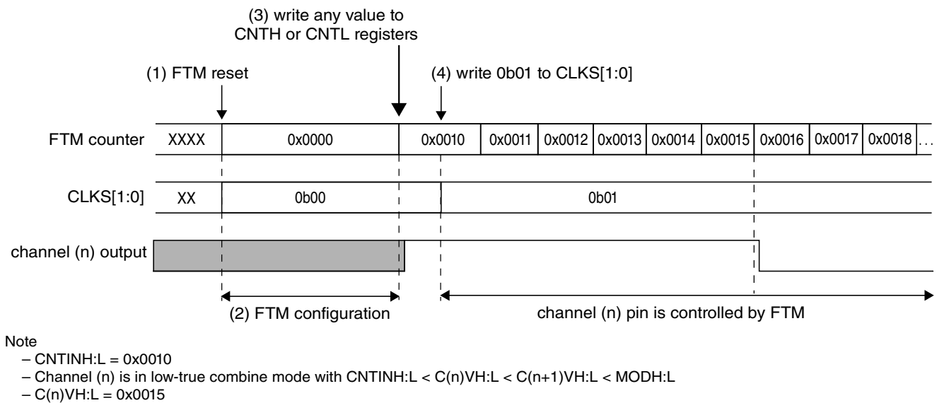
Figure 12-75. FTM behavior after the reset when the channel (n) is in combine mode
