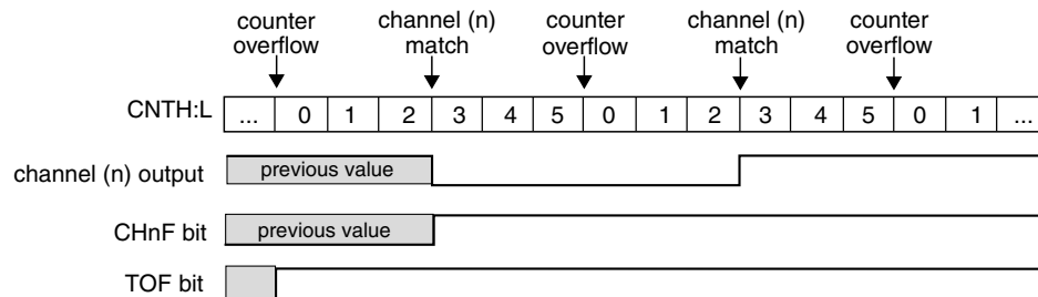
Figure 12-12. Example of the output compare mode when the match toggles the channel output
