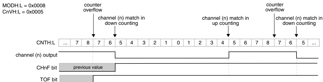
Figure 12-20. CPWM signal with ELSnB:ELSnA = X:1
