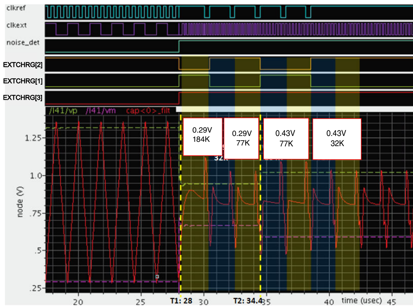
Figure 21-9. TSI noise detection mode waveform
