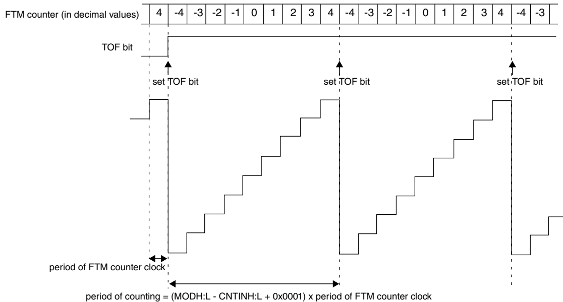
Figure 12-4. Example of FTM up and signed counting
