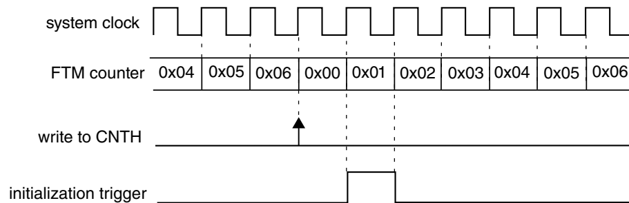
Figure 12-65. Initialization trigger is generated when there is a write to CNTH or CNTL
