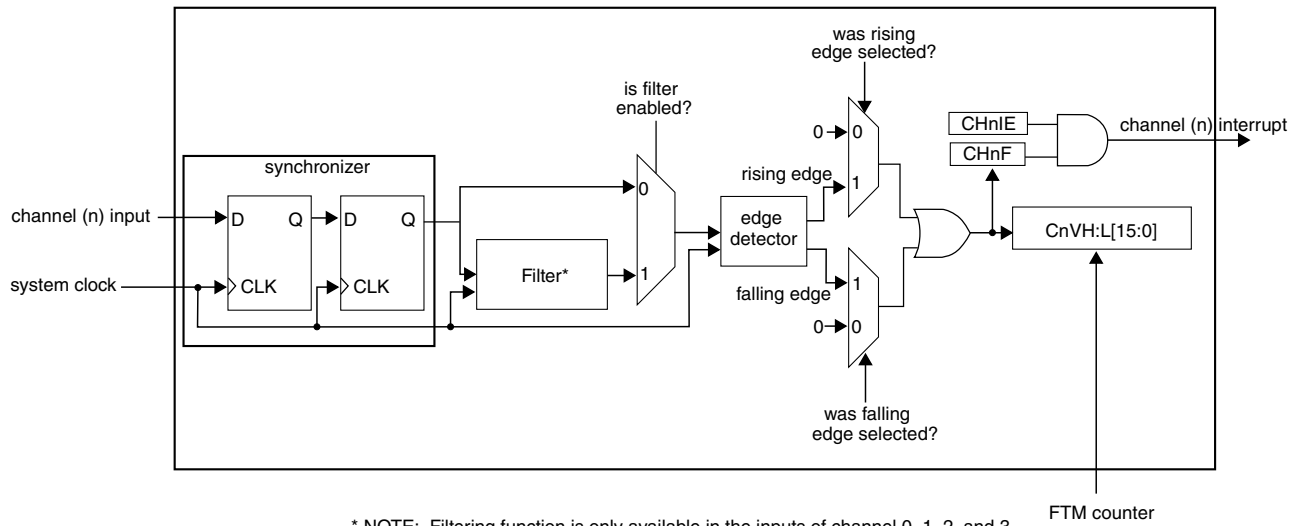
Figure 12-9. Input capture mode
