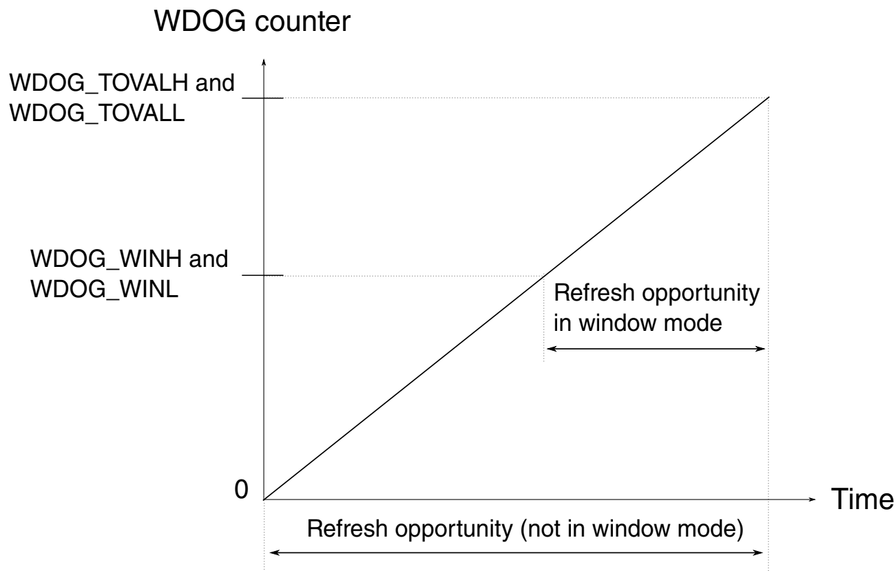
Figure 23-2. Refresh opportunity for the Watchdog counter
