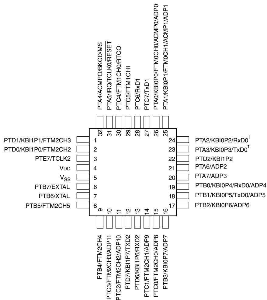
Figure 16. MC9S08PL60 32-pin LQFP package
