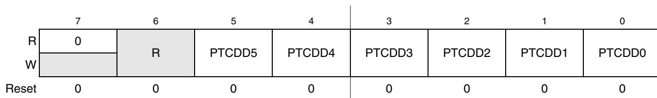
Figure 6-21. Data Direction for Port C (PTCDD) 1
