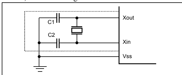
Figure 10-2 Oscillator Connections
