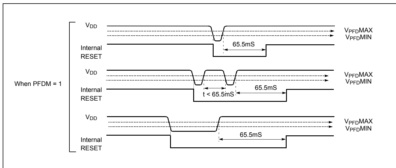
Figure 21-3 Power Fail Processor Situations (at 4MHz operation)
