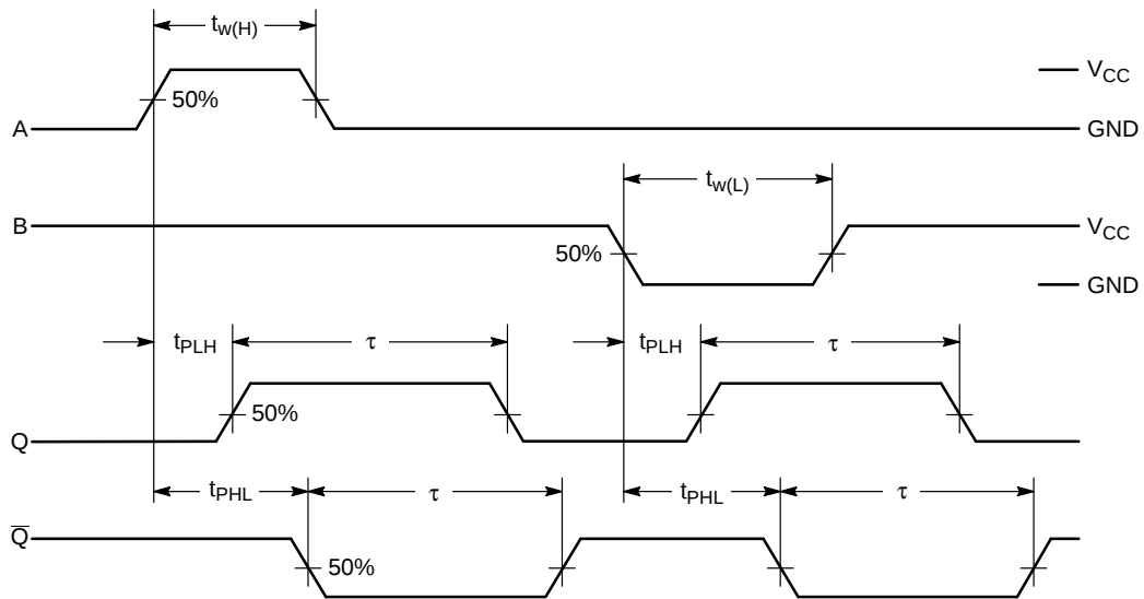
Figure 7. Switching Waveform
