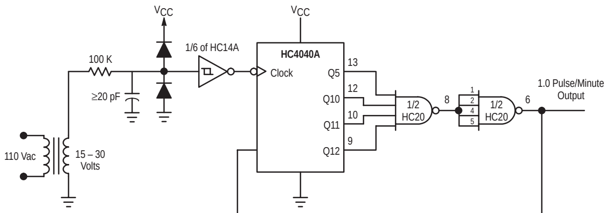
Figure 7. Time-Base Generator
