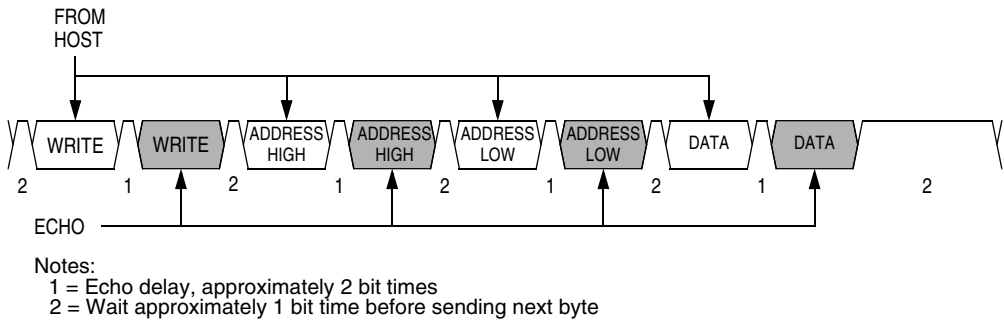
Figure 16-13. Write Transaction
