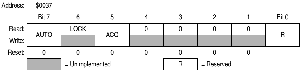
Figure 5-5. PLL Bandwidth Control Register (PBWCR)
