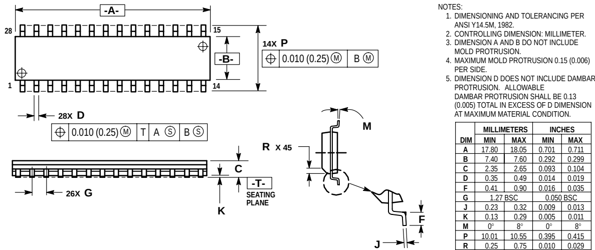
Figure 21-2. 28-Pin SOIC (Case #751F)
