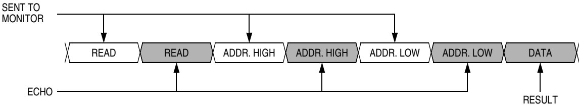
Figure 12-4. Read Transaction
