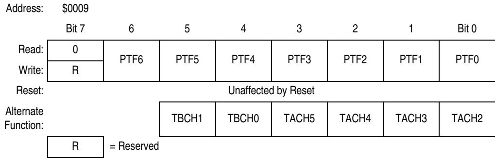
Figure 23-17. Port F Data Register (PTF)
