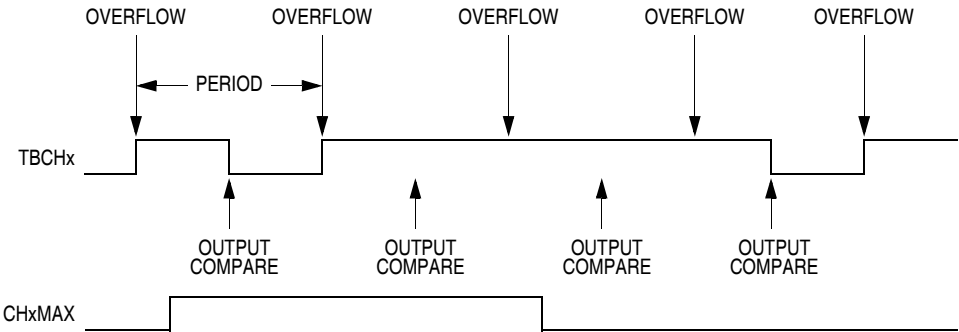
Figure 12-13. CHxMAX Latency
