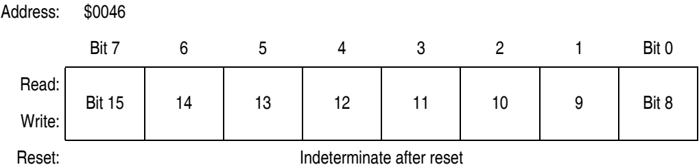
Figure 12-14. TIMB Channel 0 Register High (TBCH0H)
