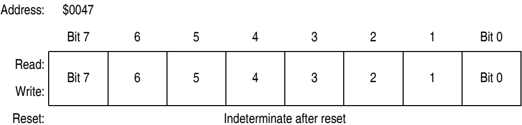
Figure 12-15. TIMB Channel 0 Register Low (TBCH0L)
