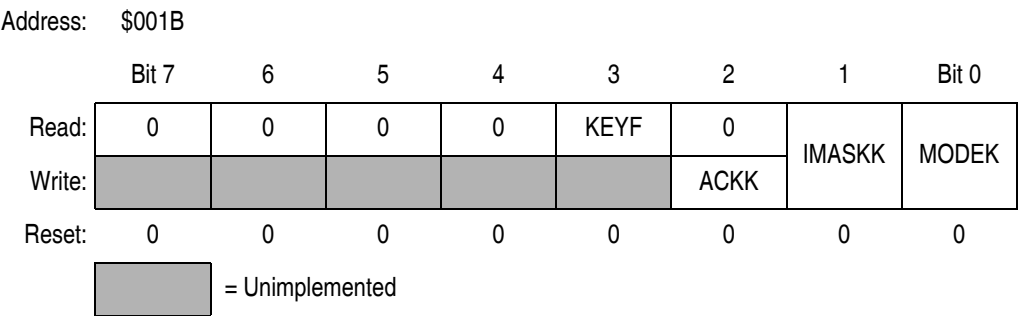
Figure 19-3. Keyboard Status and Control Register (KBSCR)
