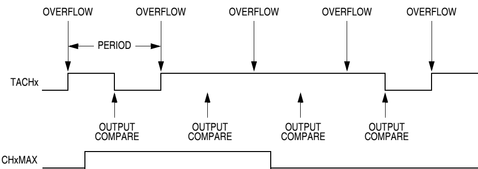
Figure 11-13. CHxMAX Latency
