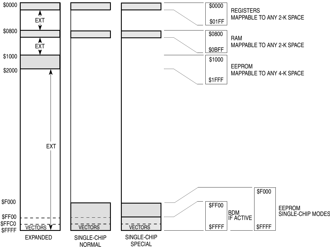
Figure 5-6. Memory Map
