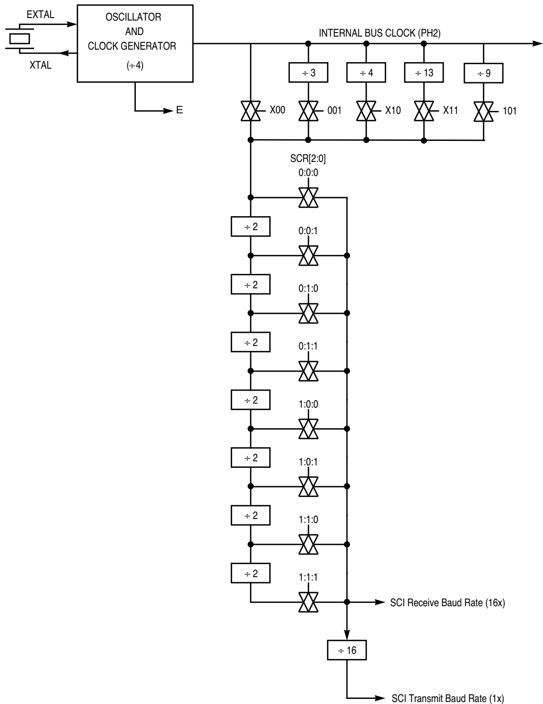
Figure 11 SCI Baud Rate Generator Block Diagram
