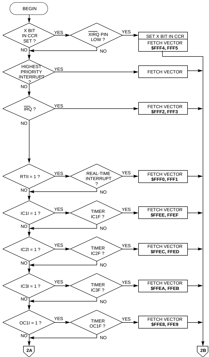
Figure 5-2 Interrupt Priority Resolution (1 of 2)
