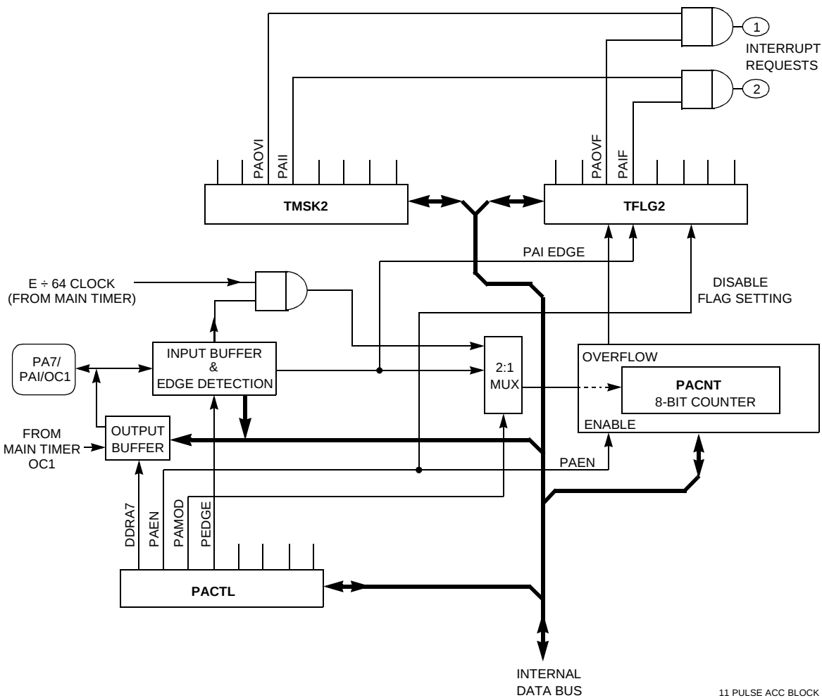
Figure 9-3 Pulse Accumulator
