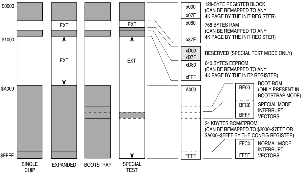
Figure 4 Memory Map
