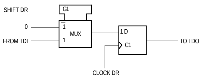
Figure 7-9. Bypass Register
