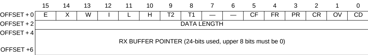
Figure 4-36. DDCMP Receive Buffer Descriptor
