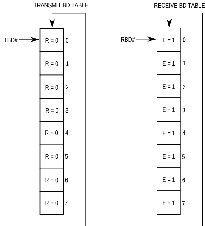
Figure D-4. Transmit and Receive BD Tables
