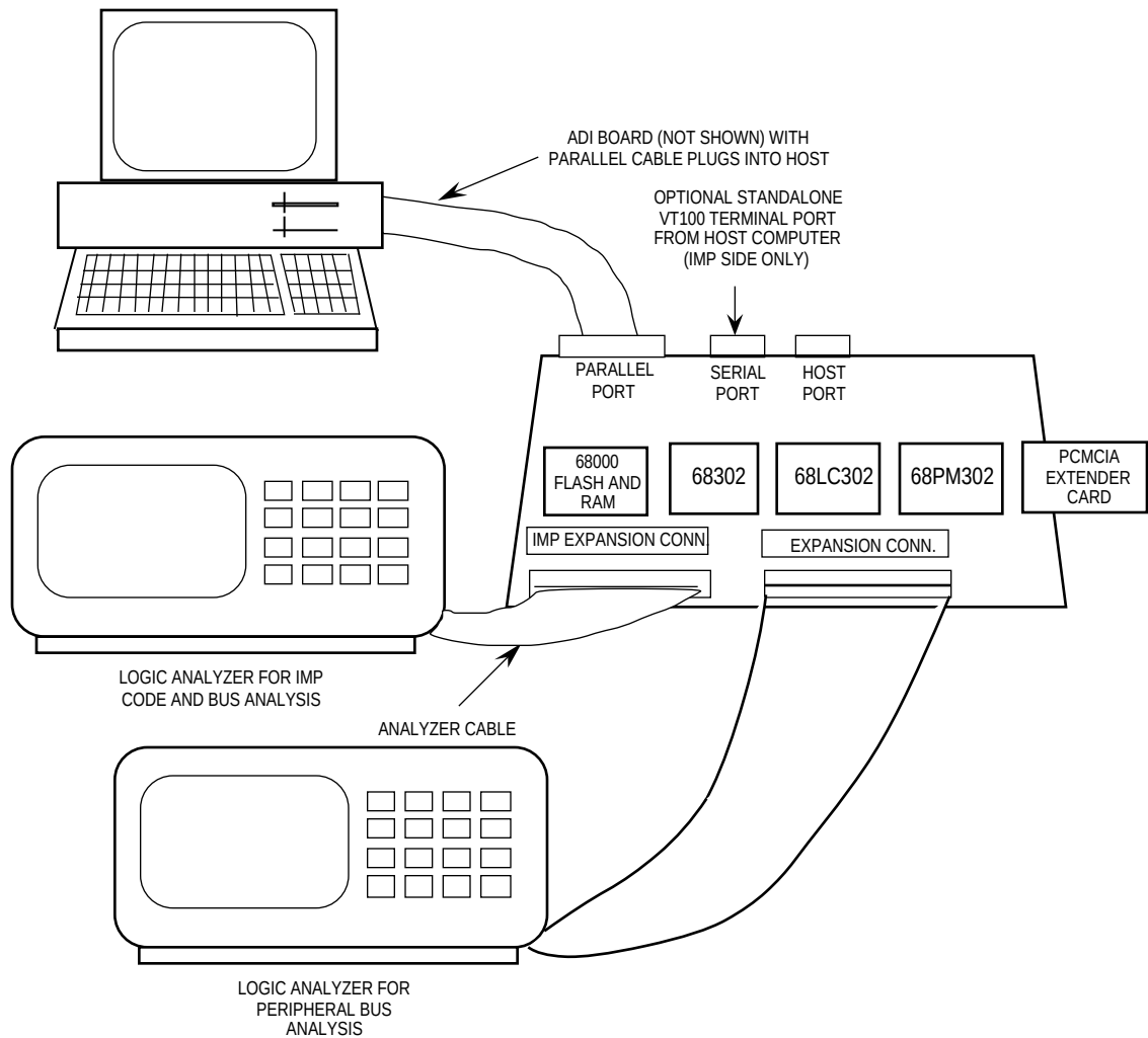
Figure 1. MC68302FADS
