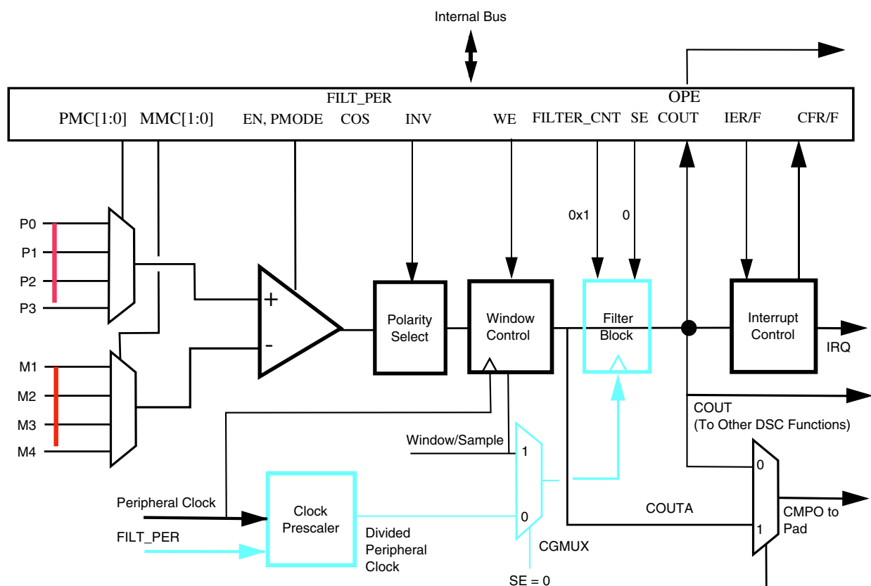
Figure 3-26. Windowed Mode
