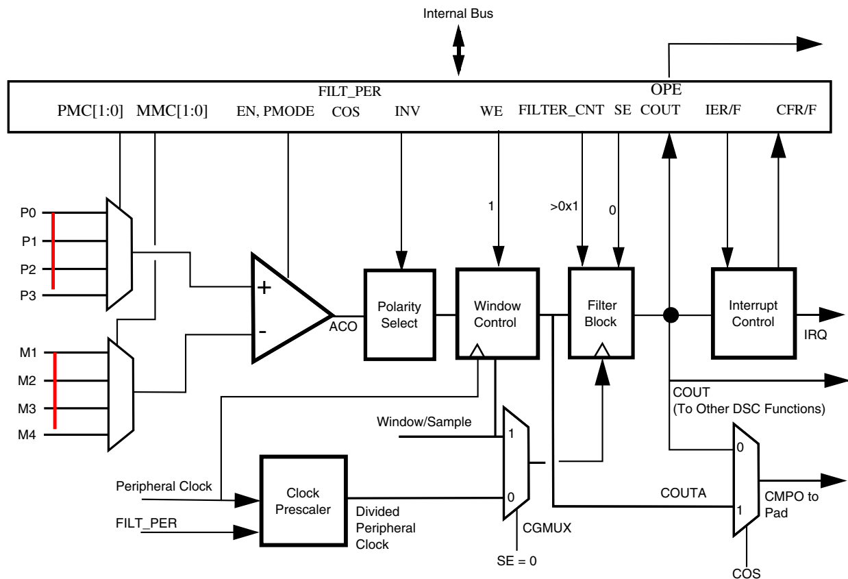
Figure 3-28. Windowed/Filtered Mode
