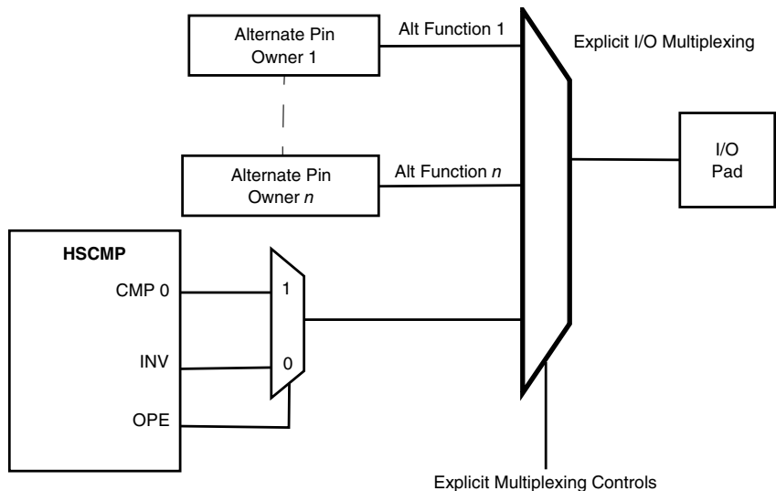
Figure 3-3. OPE Operation
