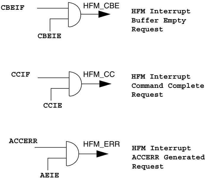
Figure 20-14. HFM Interrupt Implementation
