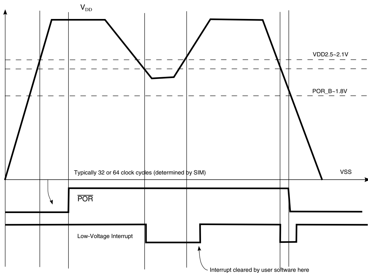
Figure 17-3. \overline{\text{POR}} Versus Low-Voltage Interrupts
