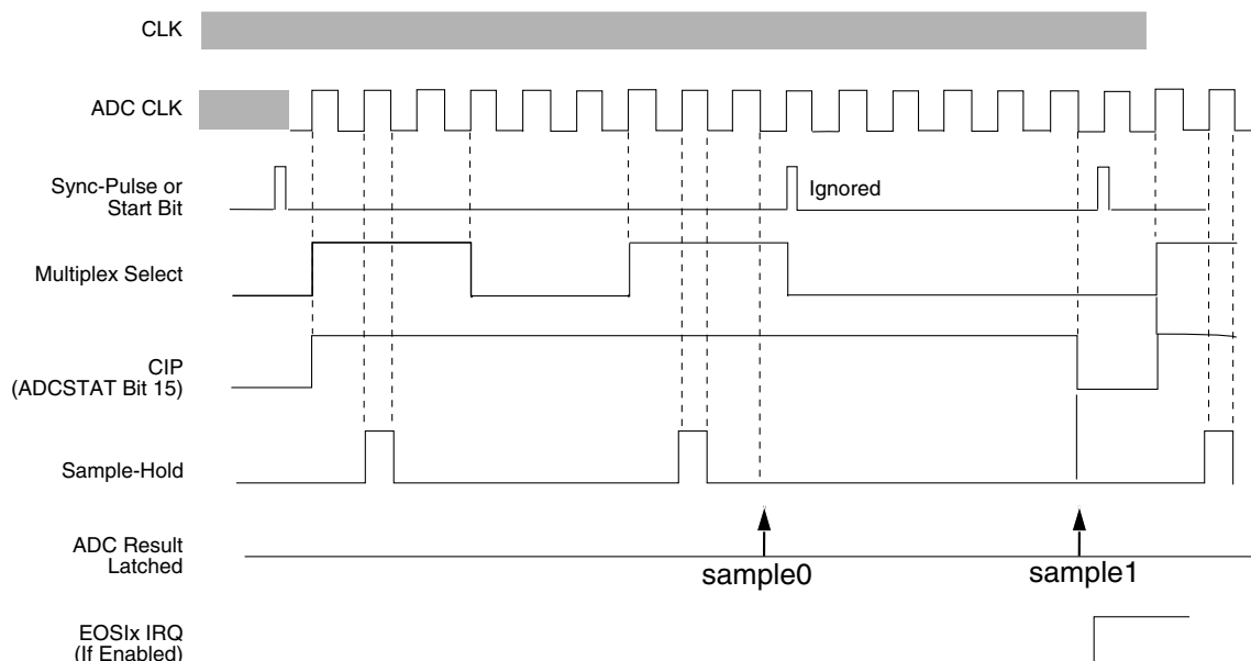
Figure 2-74. ADC Timing
