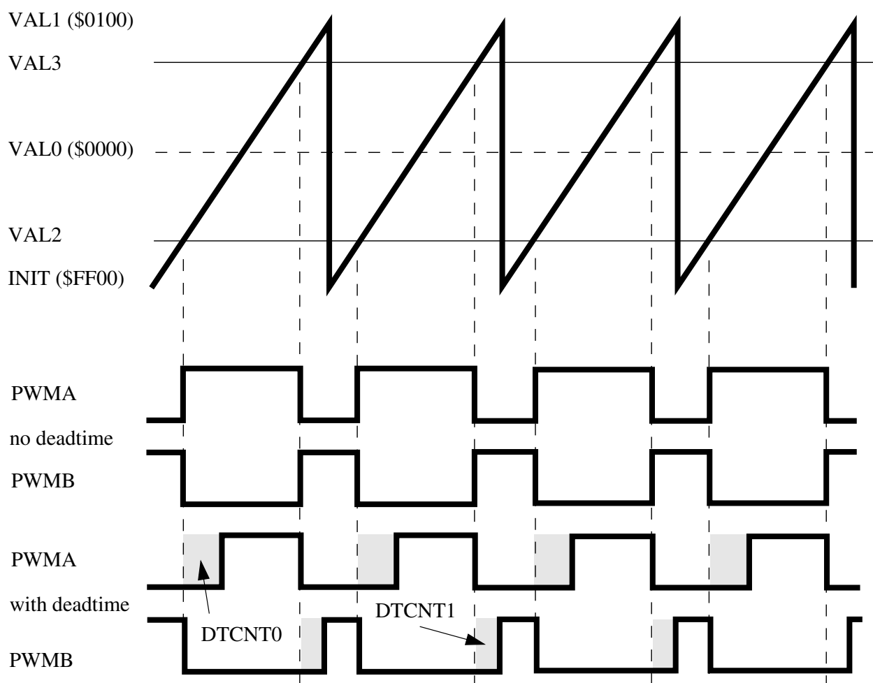
Figure 7-226. Deadtime Insertion
