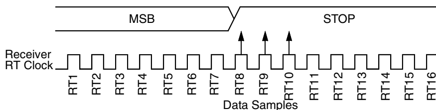
Figure 11-27. Slow Data
