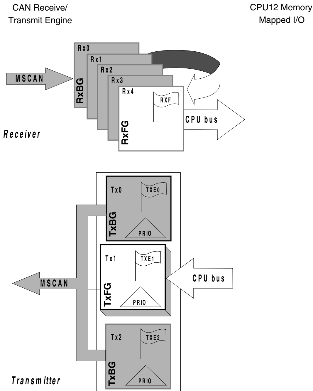
Figure 13-81. User Model for Message Buffer Organization
