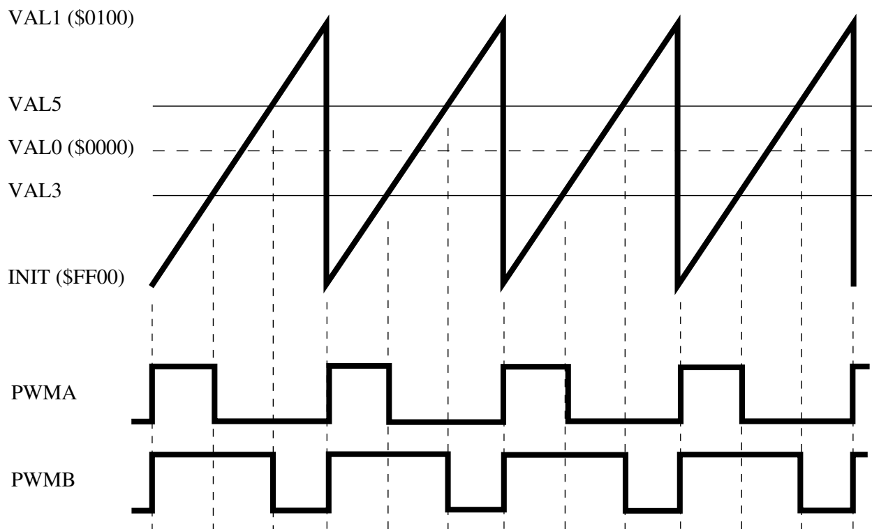
Figure 7-209. Edge Aligned Example (INIT=VAL2=VAL4)
