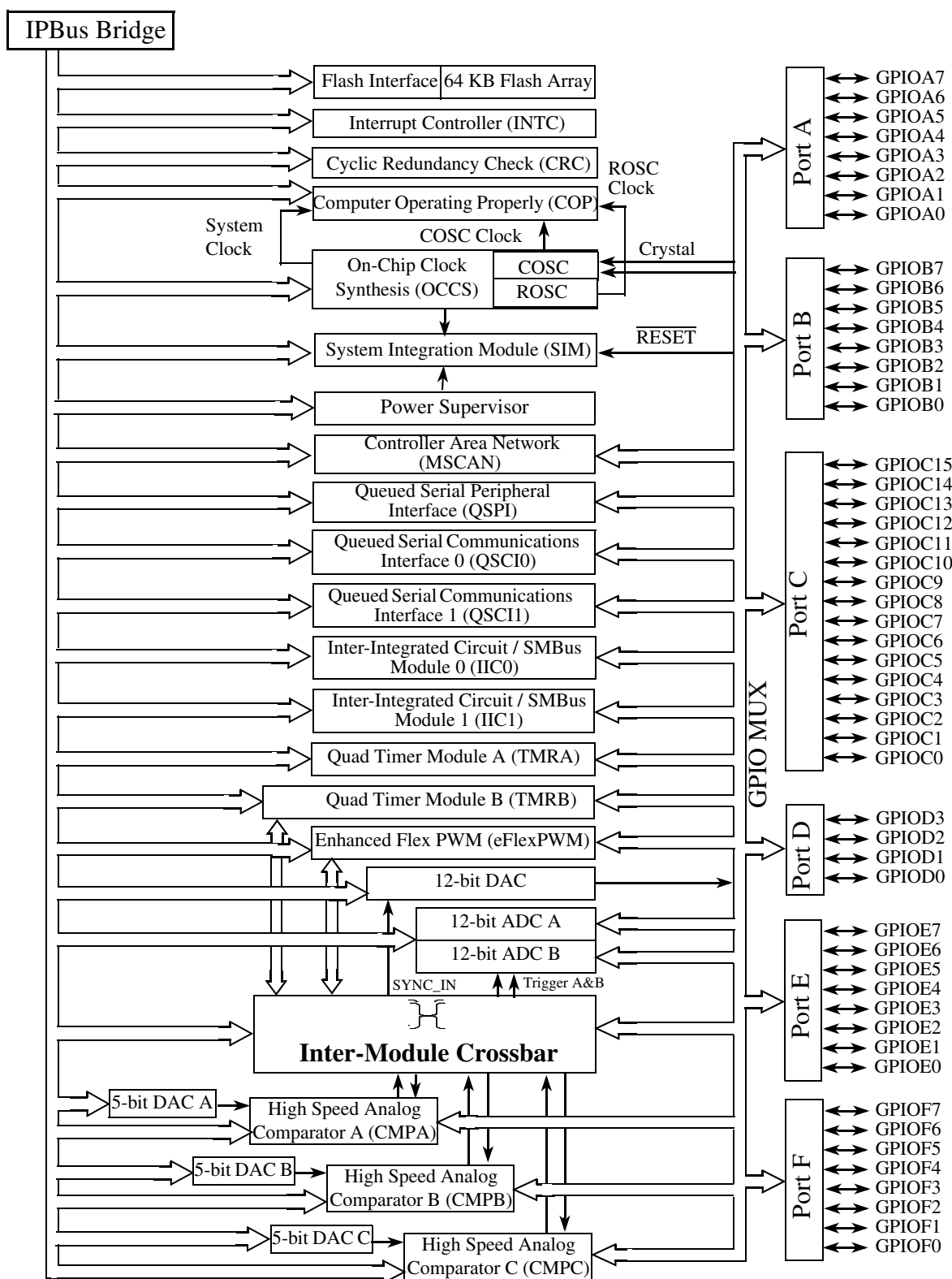
Figure 1-2. Peripheral Subsystem
