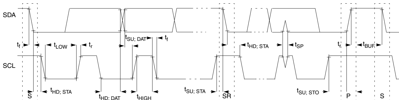
Figure 33. Timing Definition for Standard Mode Devices on the I²C Bus
