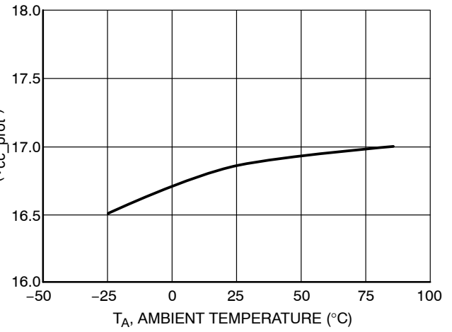
Figure 20. Protection Level on V CC vs. Temperature
