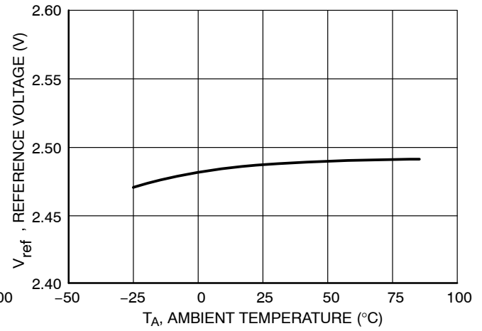
Figure 22. Reference Voltage vs. Temperature
