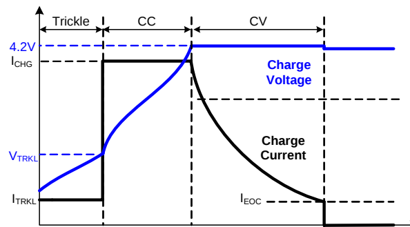
Figure 17. Charge Profile
