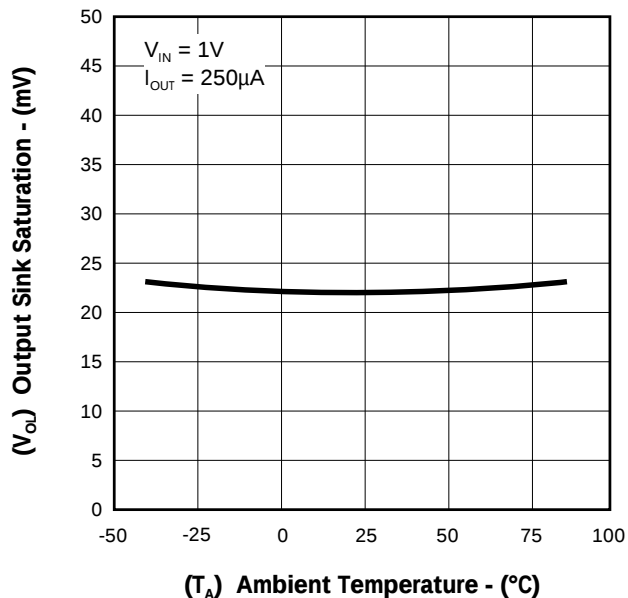
FIGURE 11. — LOW LEVEL OUTPUT SATURATION VOLTAGE vs. TEMPERATURE
