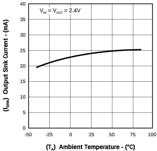
FIGURE 9. — LOW LEVEL OUTPUT CURRENT vs. TEMPERATURE
