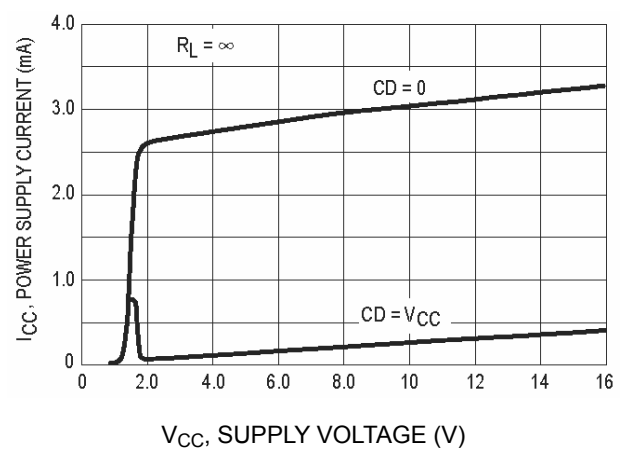
Figure 15. Power Supply Current
