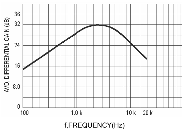
Figure 25. Frequency Response of Figure 24
