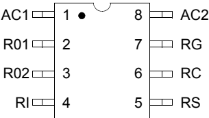
Figure 3. 34017A Terminal Connections
