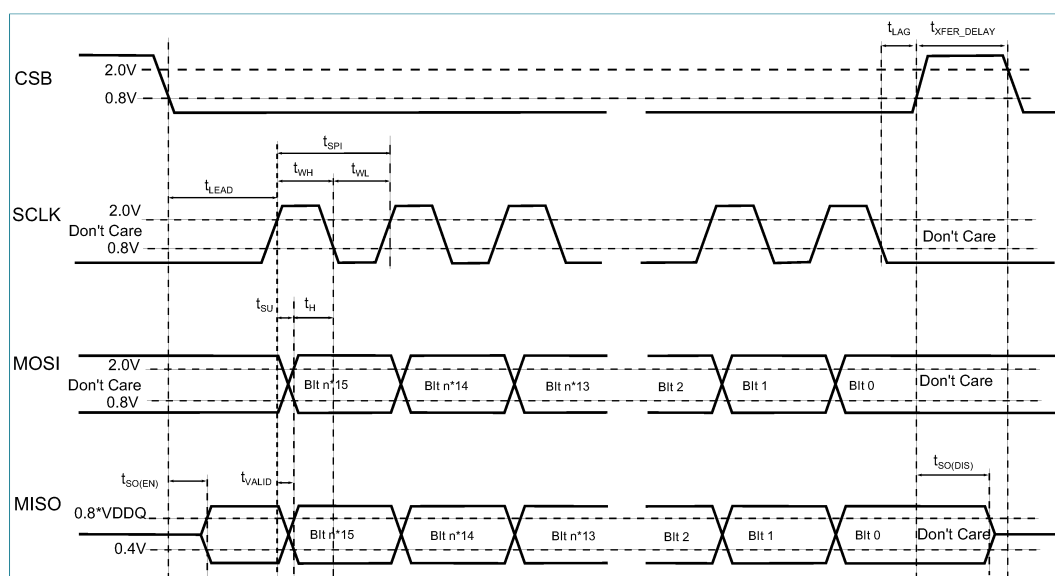
Figure 8. SPI dynamic diagram
