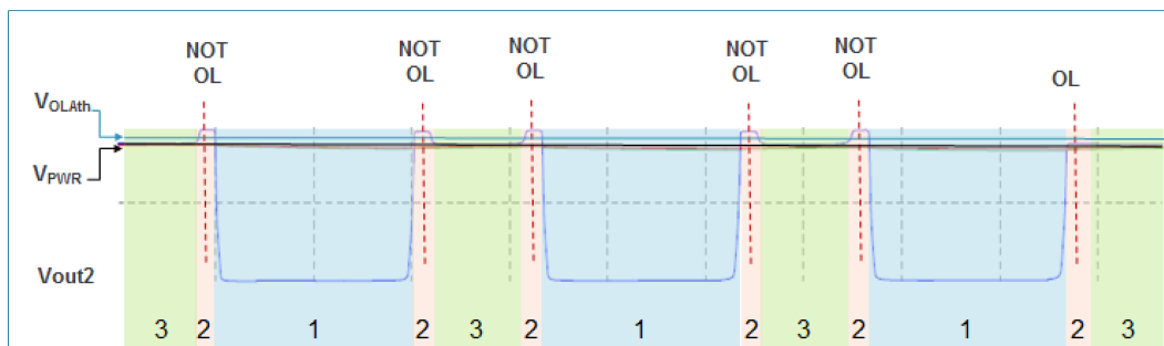
Figure 17. Open load circuit operation
