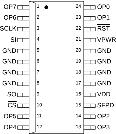
Figure 3. 33291 Pin Connections
