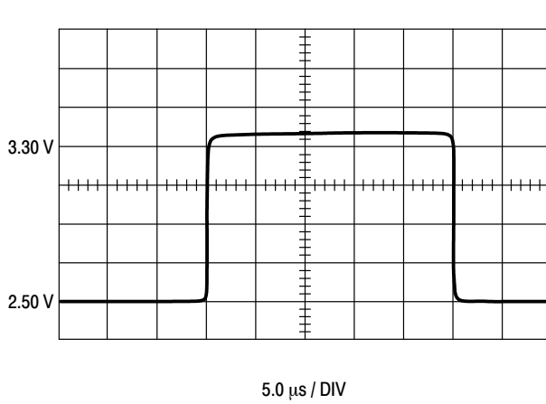
Figure 8. Error Amp Transient Response
