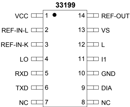
Figure 3. 33199 Pin Connections
