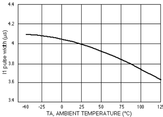
Figure 23. I1 Pulse Current Width versus Temperature
