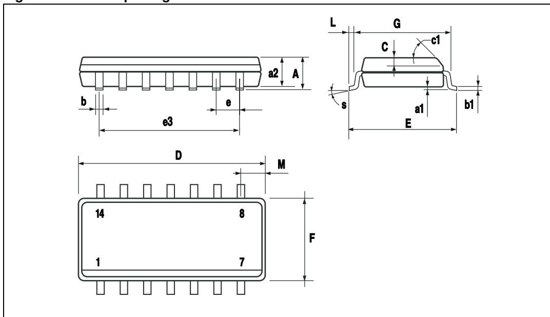
Figure 11. SO-14 package outline
