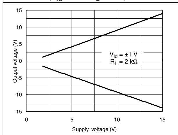
Figure 6. Output voltage vs. supply voltage ( V_{id} = \pm 1 V, R_L = 2 k \Omega )
