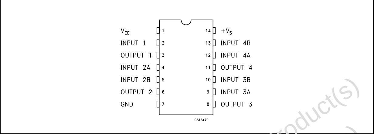
Figure 2. Pin connections
