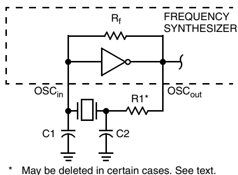
Figure 13. Pierce Crystal Oscillator Circuit
