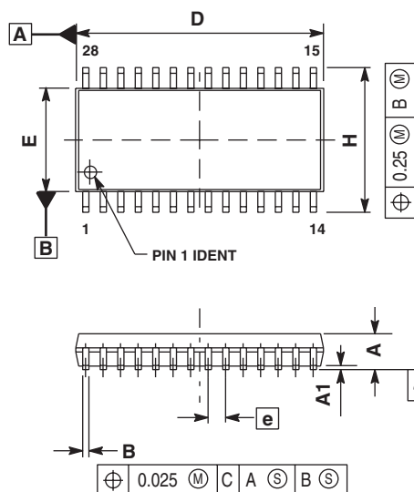
Figure 17. Outline Dimensions for SOG Package (Case Outline 751F-05, Issue F)
