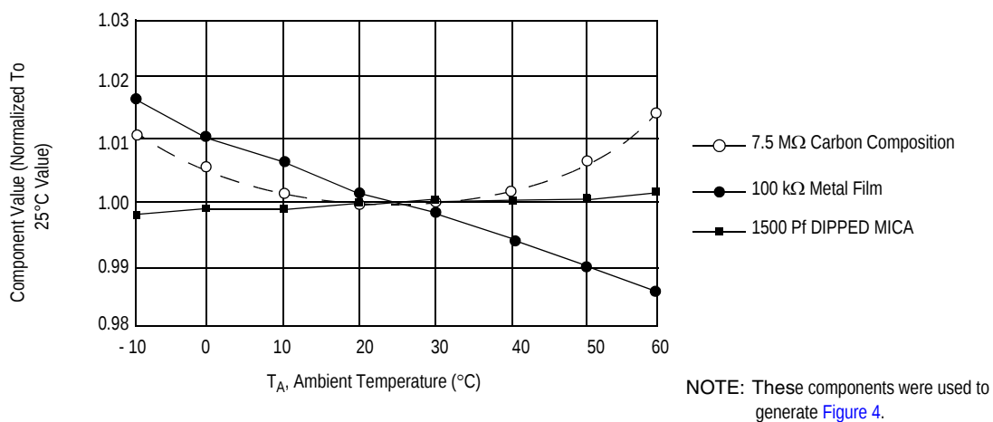
Figure 5. RC Component Variation Over Temperature
