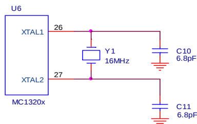
Figure 11. MC13202 Modem Crystal Circuit
