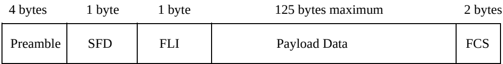
Figure 5. MC13192/MC13193 Packet Structure
