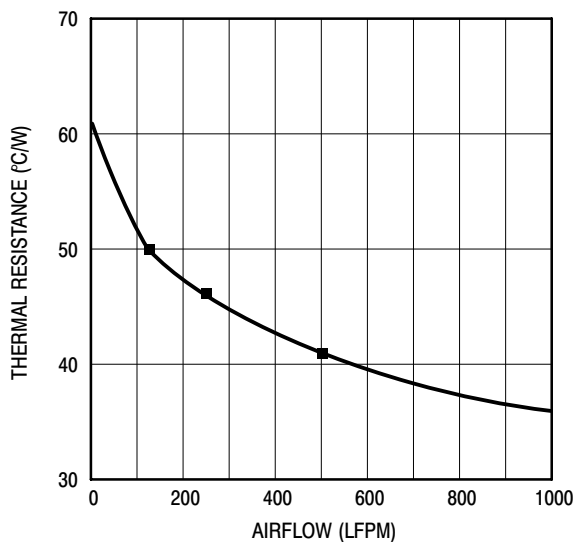
Figure 2. \theta_{JA} versus Air Flow
